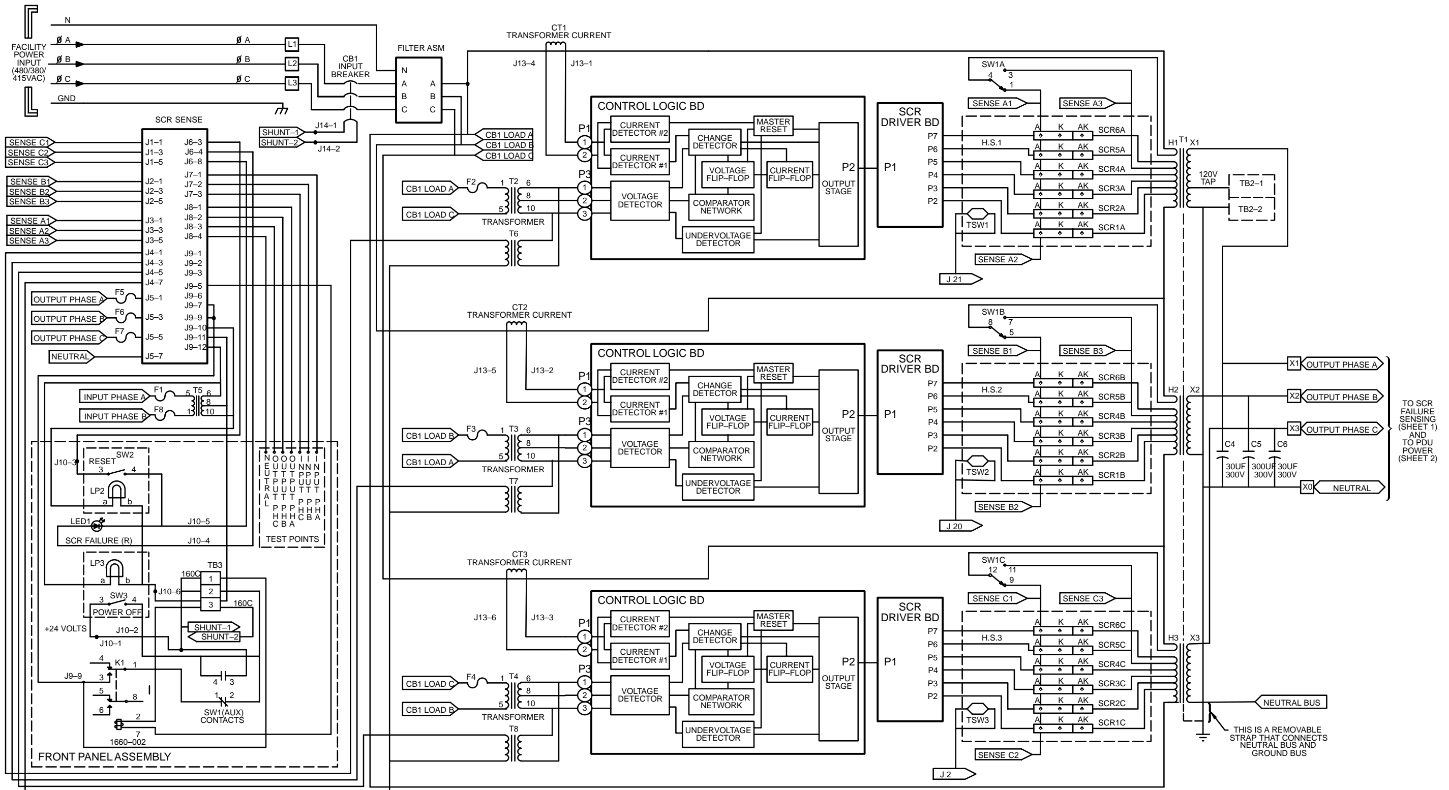
SIGNA 8.X – REGULATED COMPACT PDU
