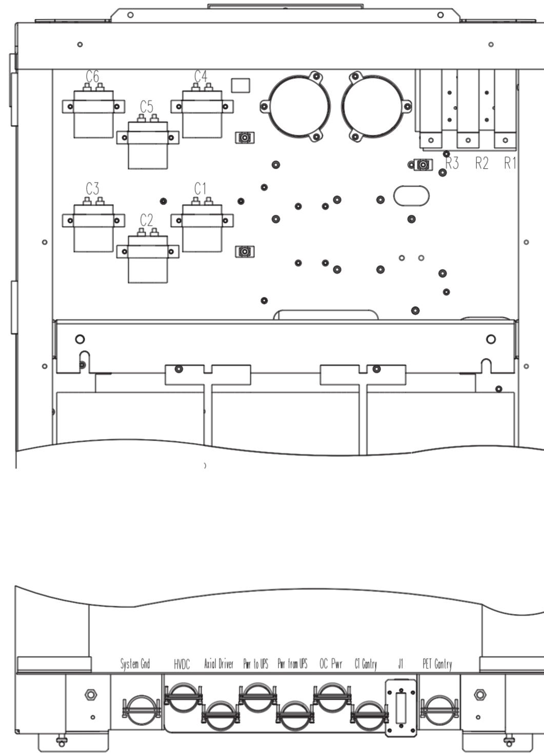
NGPDU (Cover Removed) (2326492-80)
