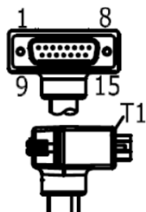
15 pin D-sub connector at J5 of CFHC (5428364)
