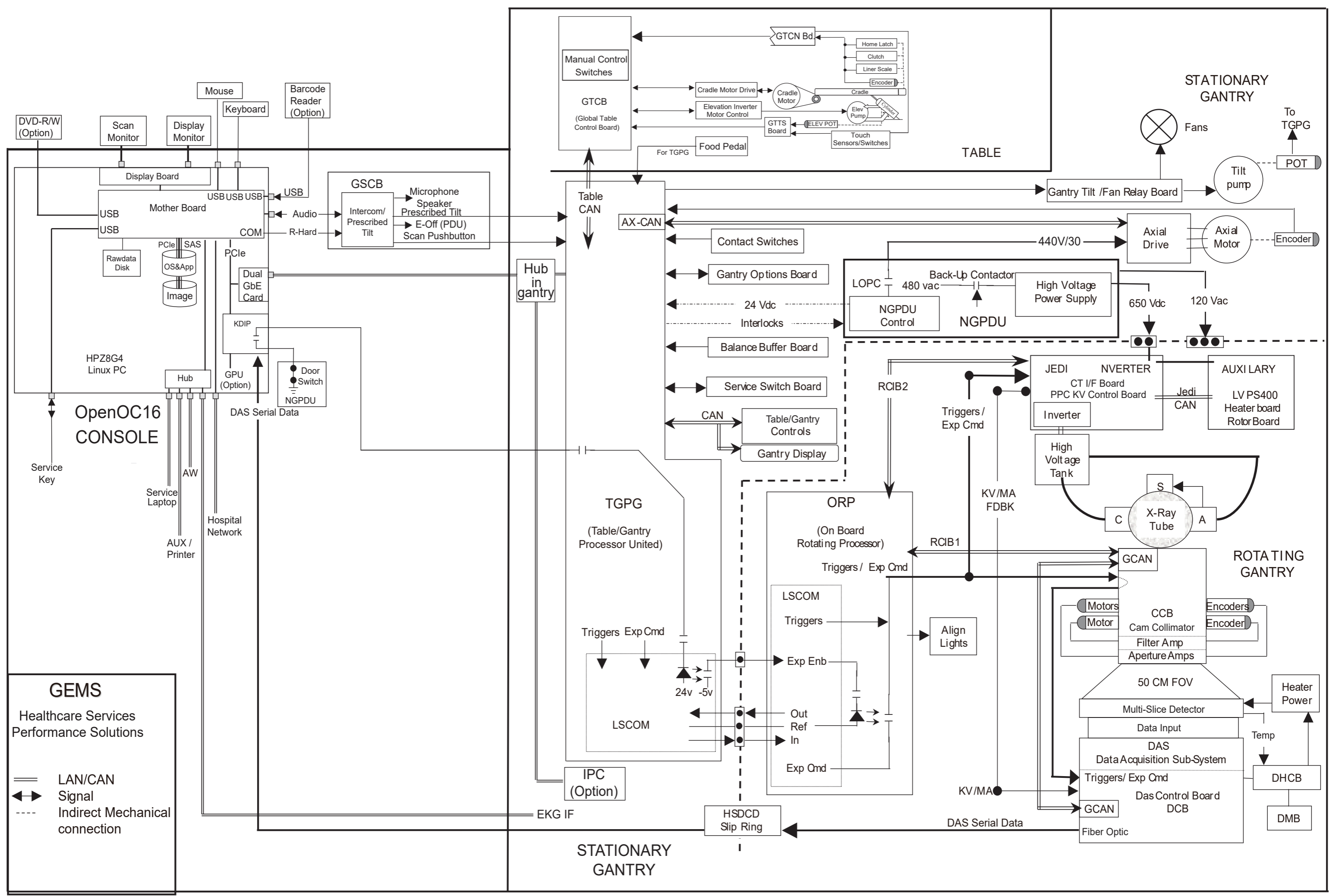
Optima CT540 with OpenOC16 (Z8G4) System Block Diagram
