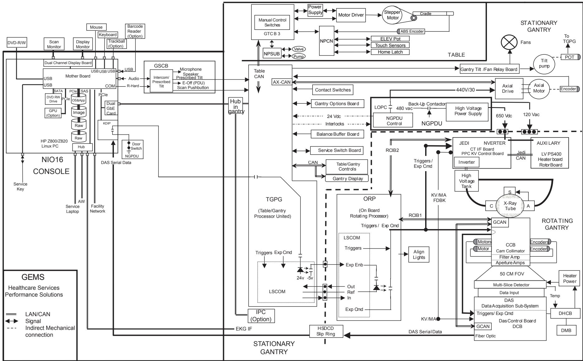
Optima Elite System Block Diagram
