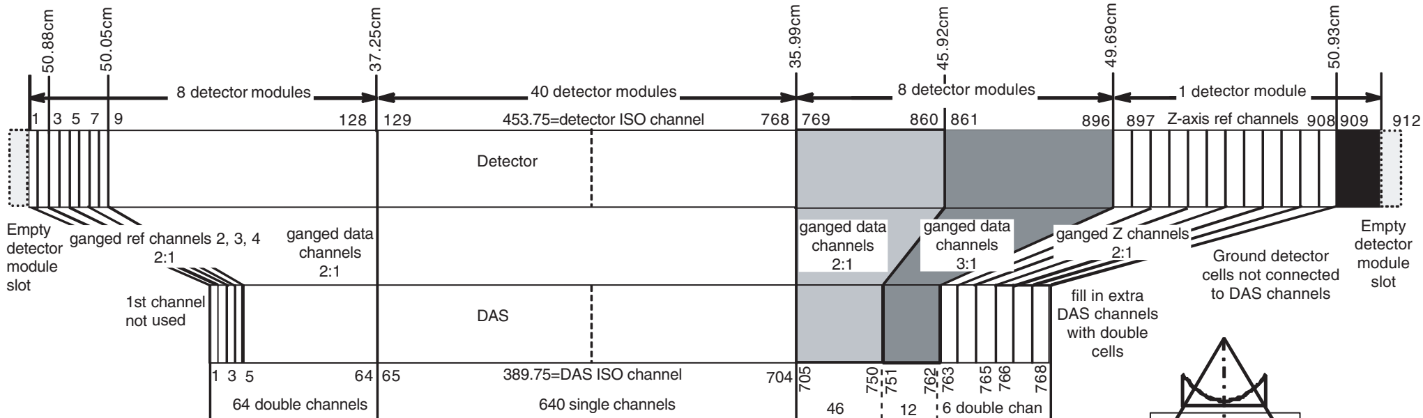
Warp 3 Detector to Das Architecture Channel Map (Same as Lightspeed QXI with "50cm DFOV, Except Z-ref cells are 2:1 instead of 4:1)
